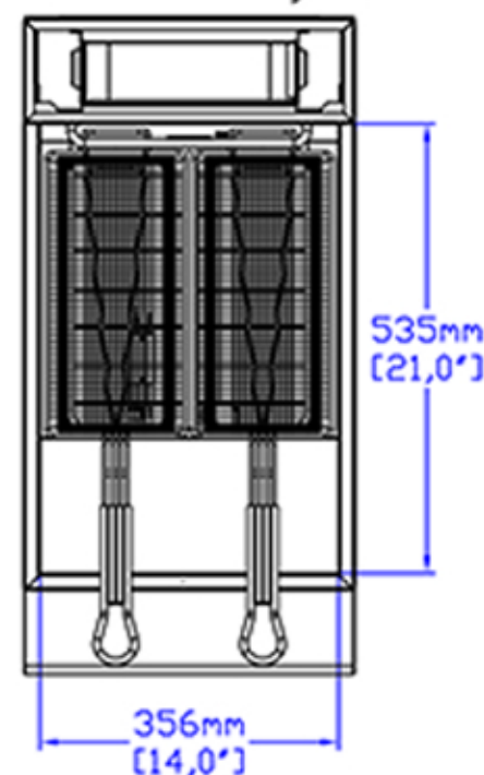
3 tube Fryer
